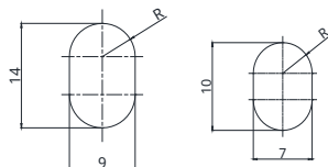
Mounting Hole
